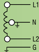
Split Phase 3 Wire + Ground
